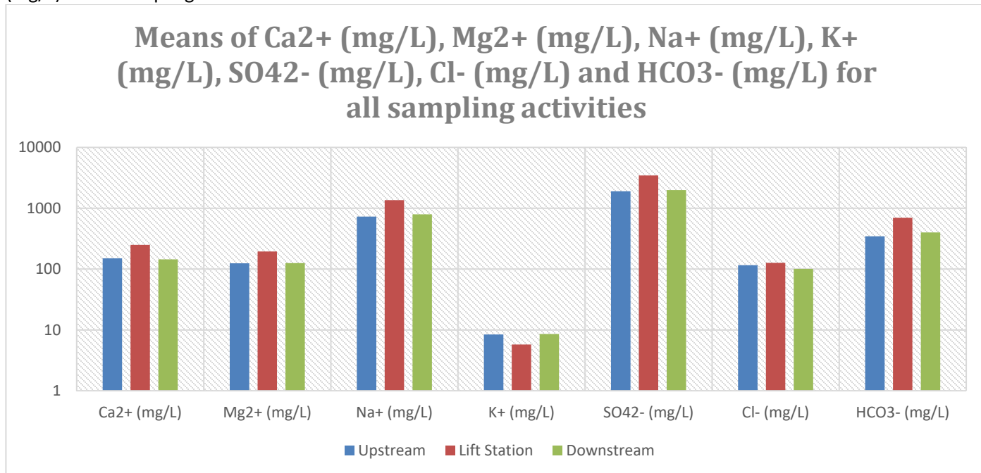
Figure 28. Cumulative means of Ca 2+ (mg/L), Mg 2+ (mg/L), Na + (mg/L), K + (mg/L), SO 4 2- (mg/L), Cl - (mg/L) and HCO 3 - (mg/L) for all sampling activities.
